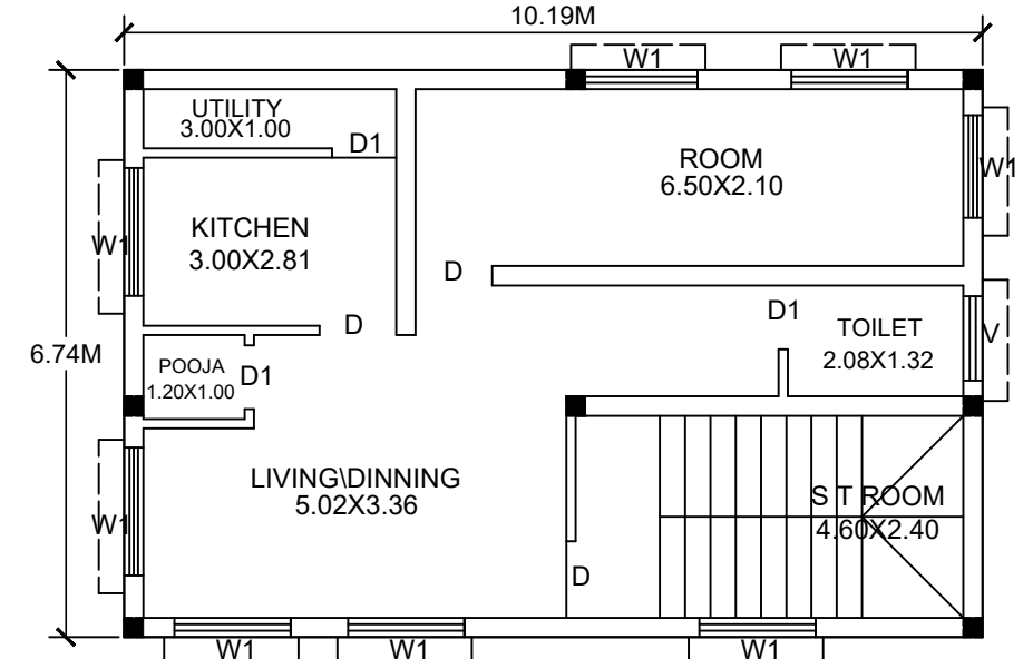
PROPOSED TYPICAL FIRST & SECOND FLOOR PLAN
