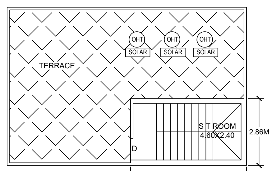
PROPOSED TERRACE FLOOR PLAN
